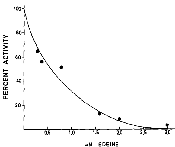
Fig.1. Effect of edeine on exogenous messenger translation in the whole wild-type lysate system. Incubations were carried out as described in the text. Edeine (Calbiochem Behring, La Jolla, CA) was added prior to the messenger. The results are expressed as percent activity obtained in the presence of edeine as compared to controls in the absence of the antibiotic. 100% corresponded to 532128 cpm. Data have been corrected for endogenous mRNA radioactivity incorporation by subtracting it (22320 cpm) from the [ ^3 H]leucine incorporated in the presence of exogenous mRNA.
